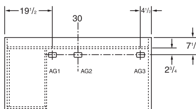
30 x 60 single pedestal left desks ( 3060SPL )
